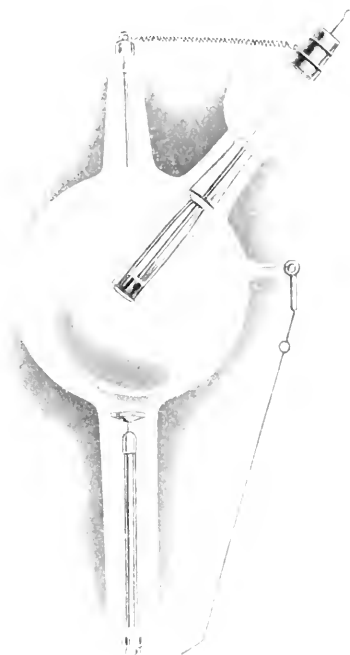
FIG. 28.—Water-cooled tube arranged for overhead work. (C. Andrews.)
